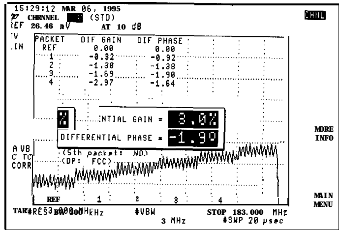
Figure g-15. Differential Gain/Differential Phase
